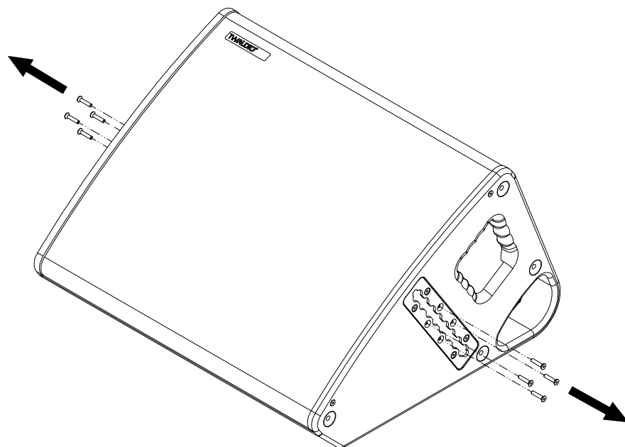
Figure 4.4.1 - Removing the countersunk screws on the C15 loudspeaker
