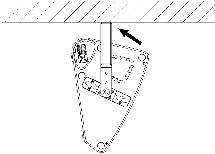
Figure 4.5 - Assembly QBC15 with C15 to ceiling
