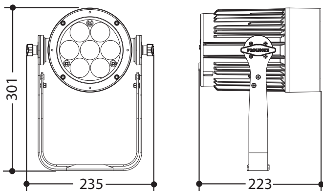
Technical drawing
