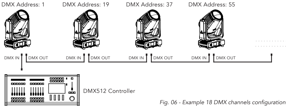
Fig. 06 - Example 18 DMX channels configuration
