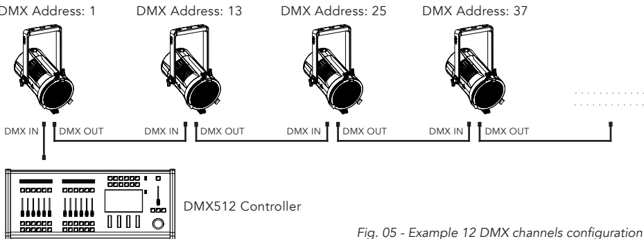
Fig. 05 - Example 12 DMX channels configuration
