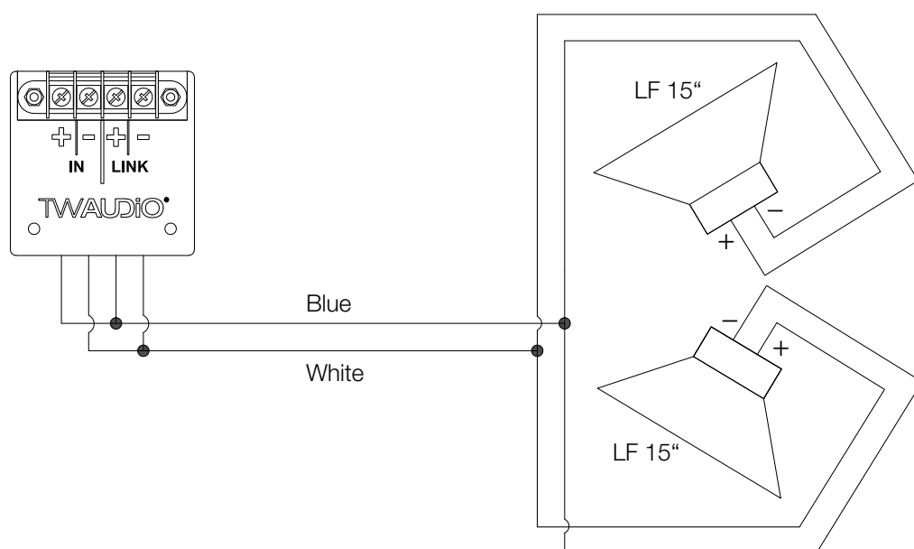
Figure 3.2 - Connection diagram
